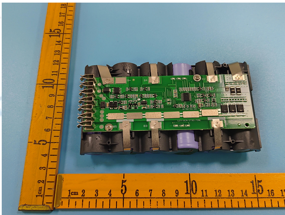
Fig.4 Internal view of Lithium-ion Battery Pack 锂离子电池组内部
