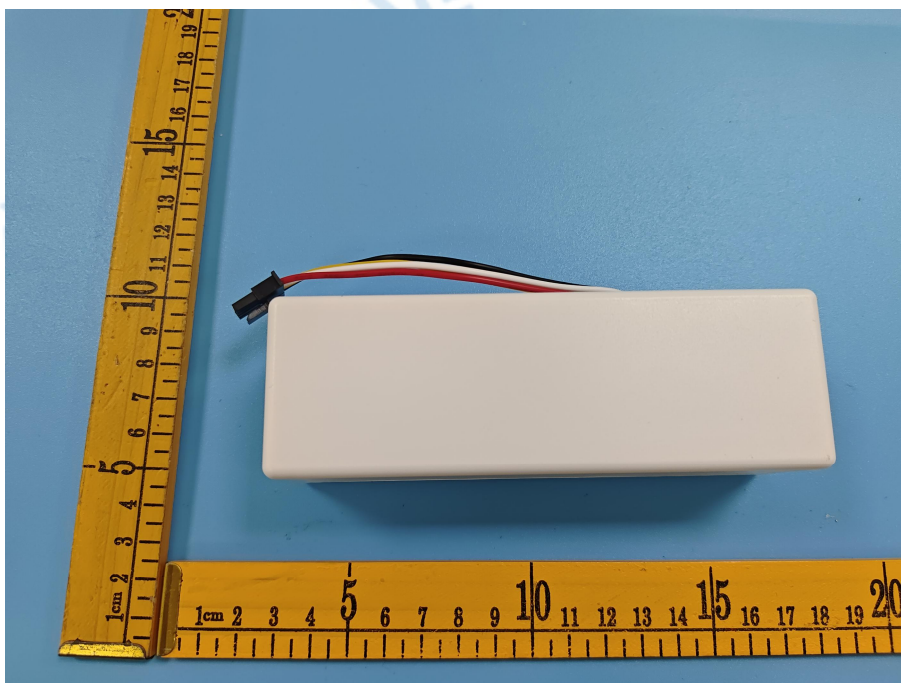
Fig.2 Back view of Lithium-ion Battery Pack 锂离子电池组背面
