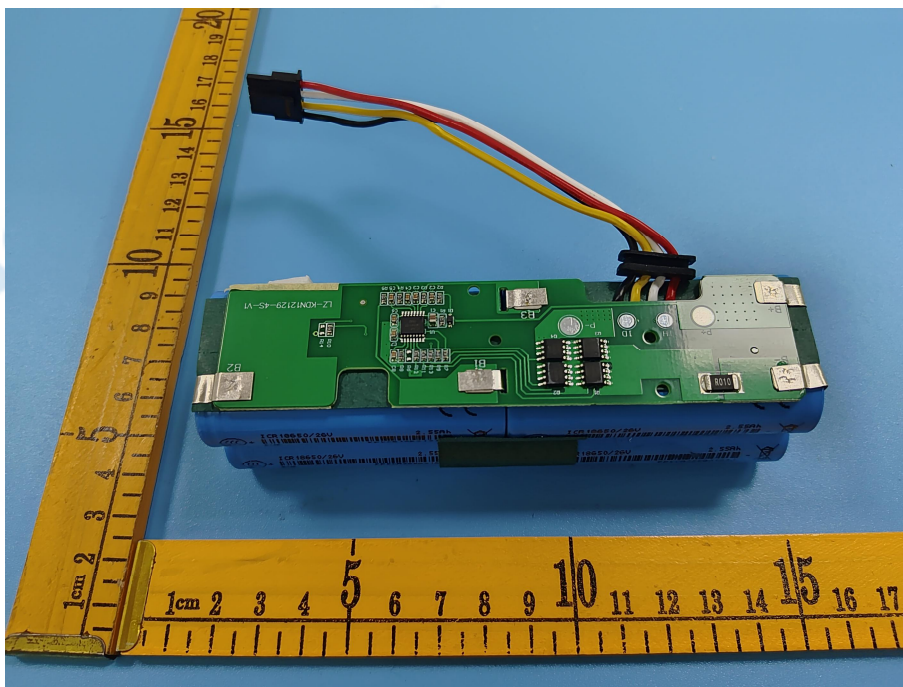
Fig.3 Internal view of Lithium-ion Battery Pack 锂离子电池组内部
